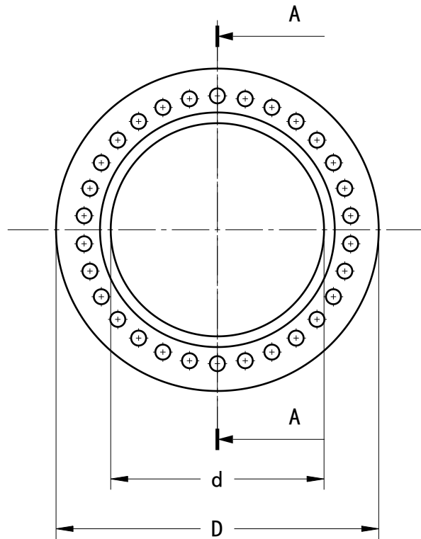
Front view Scale: 2:1
