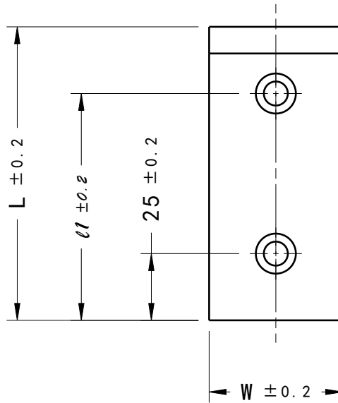
Hole type A
