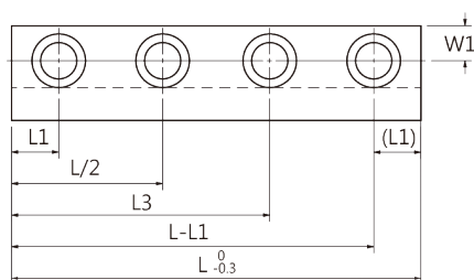
4處安裝螺栓孔 Mounting bolt hole:4
