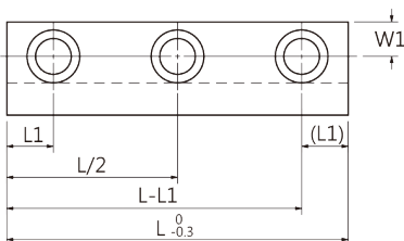
3處安裝螺栓孔 Mounting bolt hole:3
